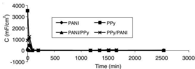
Fig. 15. C_{m/p} , capacitance of metal/polymer interface in 0.1 M NaCl solution during immersion times
