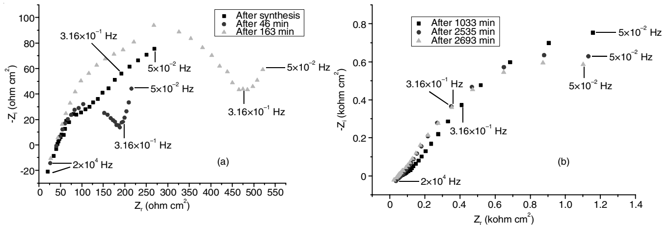
Fig. 11. (a-b) Nyquist plots for the corrosion of PANI/PPy covered mild steel in 0.1 M NaCl solution measured after various exposure times
