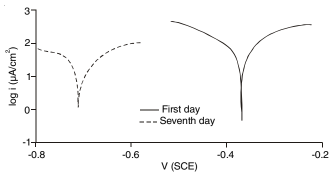
Fig. 7. Tafel plots for PPy/PANI coated mild steel in 0.1 M NaCl solution
