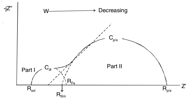
Fig. 2. Model Nyquist plot used to find R_s , C_{mp} , R_{Fe} , C_{p/e} , R_{mp} values
