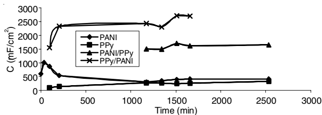
Fig. 18. C_{\text{p/e}} for coated steel during immersion in 0.1 M NaCl solution
