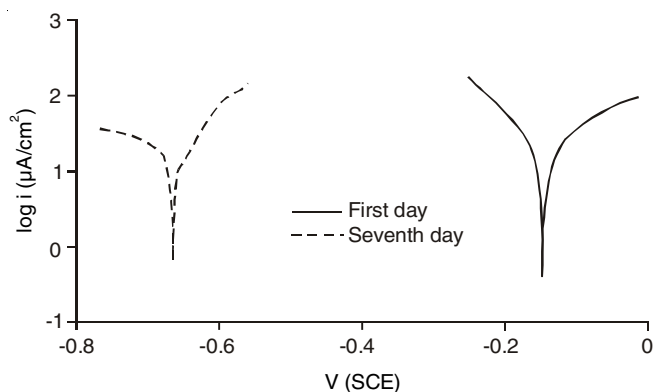
Fig. 5. Tafel plots for PPy coated mild steel in 0.1 M NaCl solution
