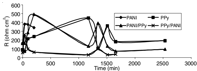
Fig. 14. R_{Fe} , corrosion resistance of mild steel between metal/polymer interface in 0.1 M NaCl solution during immersion times
