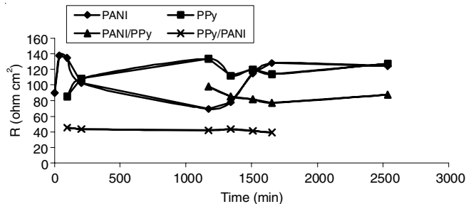
Fig. 16. R_{\text{film}} for coated steel during immersion in 0.1 M NaCl solution
