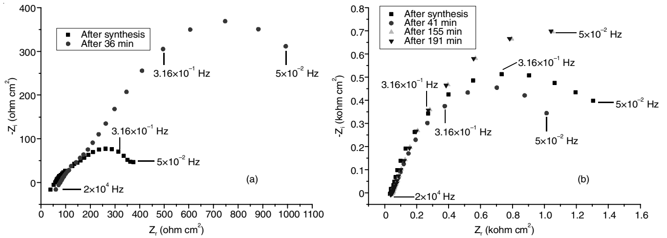
Fig. 9. (a-b) Nyquist plots for the corrosion of PANI covered mild steel in 0.1 M NaCl solution measured after various exposure times
