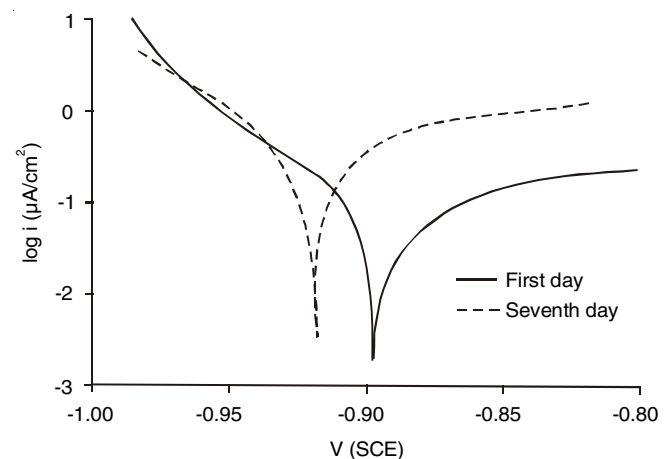
Fig. 3. Tafel plots for bare steel in 0.1 M NaCl solution
