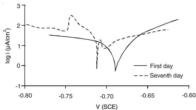
Fig. 6. Tafel plots for PANI/PPy coated mild steel in 0.1 M NaCl solution
