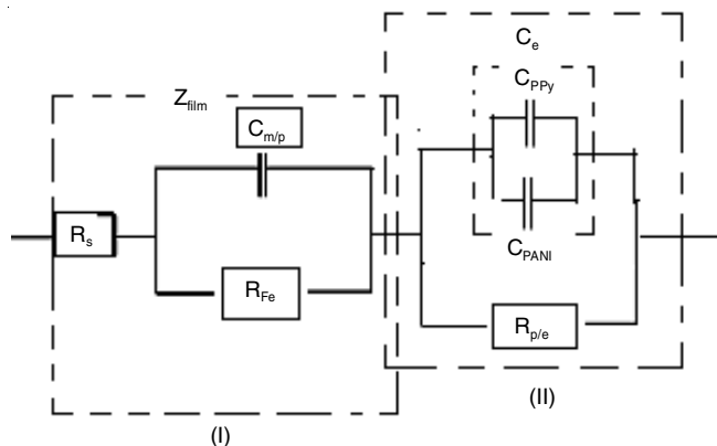
Fig. 1. Equivalent circuit considered for the corrosion of PANI or PPy or PPy/PANI or PANI/PPy coated mild steel in 0.1 M NaCl solution. For composite coatings, C_e represents equivalent capacitance of composites
