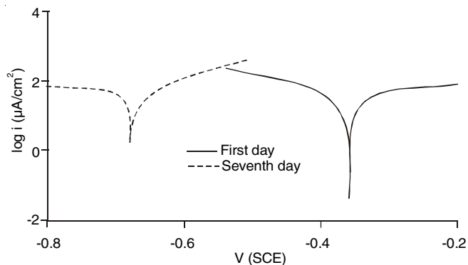
Fig. 4. Tafel plots for PANI coated mild steel in 0.1 M NaCl solution
