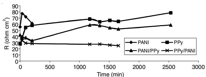
Fig. 13. R_s , resistance of the solution during the immersion times of coated steel in 0.1 M NaCl solution
