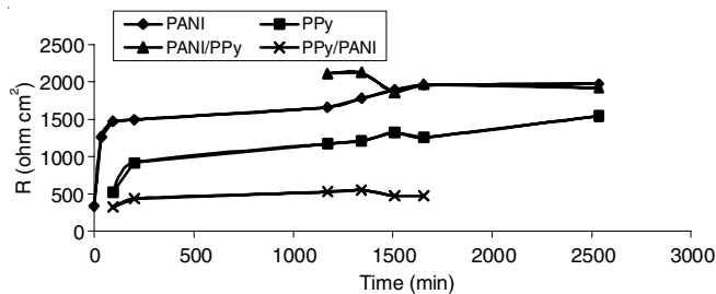
Fig. 17. R_{\text{p/e}} for coated steel during immersion in 0.1 M NaCl solution
