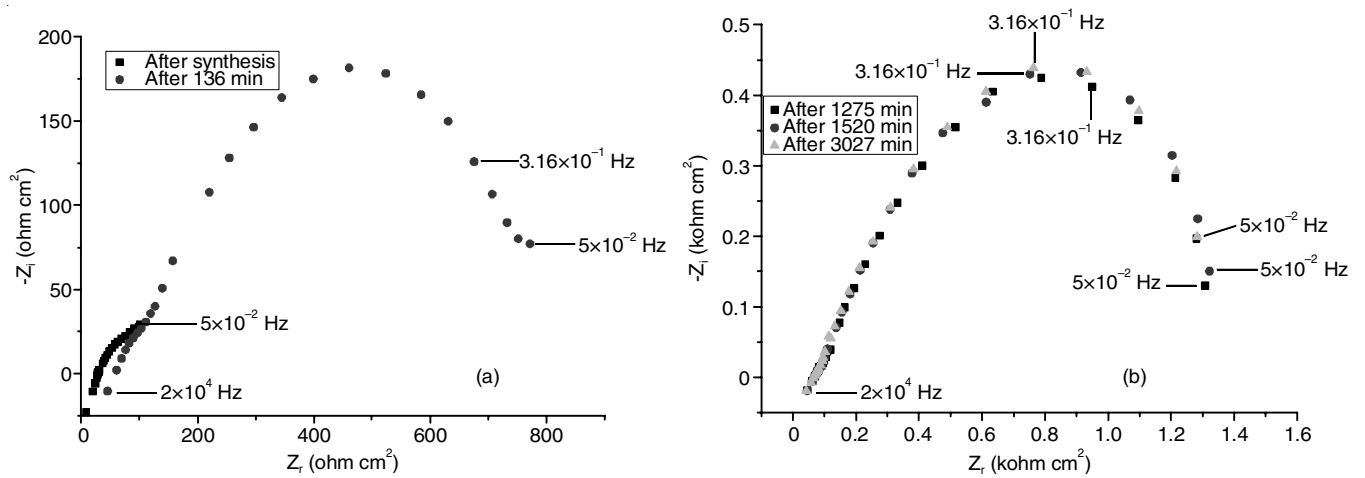
Fig. 10. (a-b) Nyquist plots for the corrosion of PPy covered mild steel in 0.1 M NaCl solution measured after various exposure times
