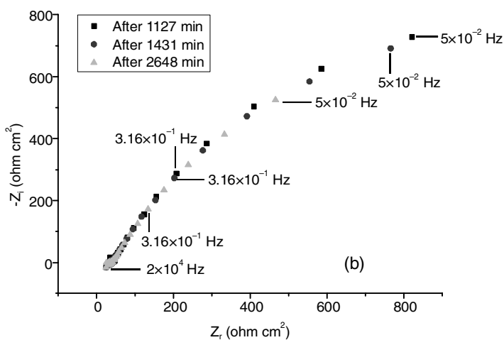
Fig. 8. (a-b) Nyquist plots for the corrosion of bare steel in 0.1 M NaCl solution measured after various exposure times
