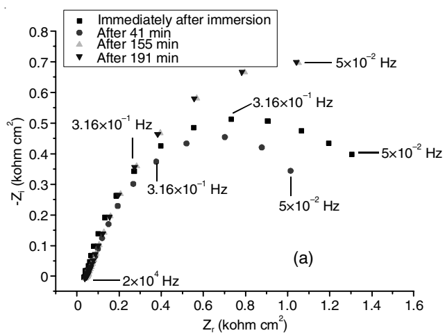
Fig. 8. (a-b) Nyquist plots for the corrosion of bare steel in 0.1 M NaCl solution measured after various exposure times
