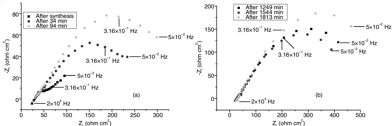
Fig. 12. (a-b) Nyquist plots for the corrosion of PPy/PANI covered mild steel in 0.1 M NaCl solution measured after various exposure times
