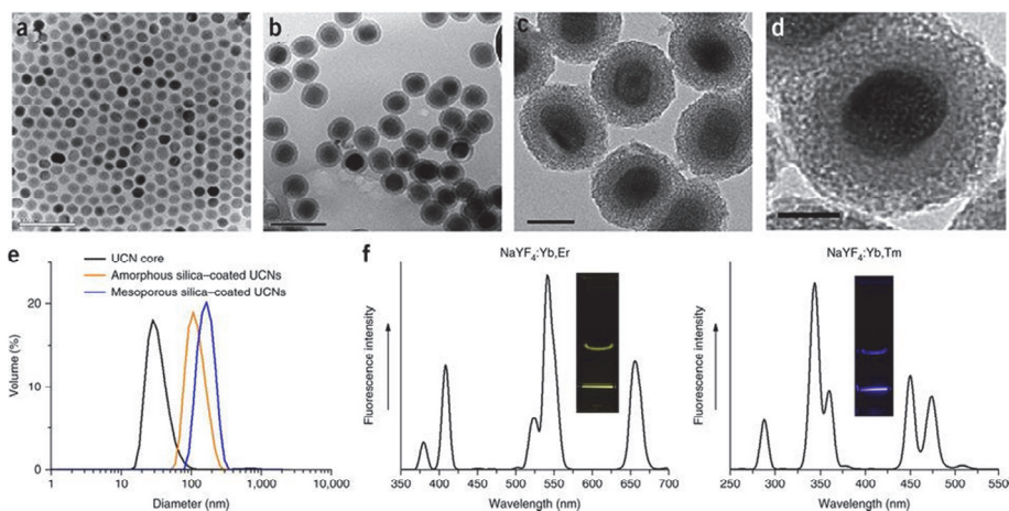
Figure 3.8.2: a) UCNC core structure, b) amorphous silica coated UCNCs, TEM images of mesoporous silica coated UCNCs c) in 50 nm and d) in 25 nm [Gnanasammandhan et al. 2016].
