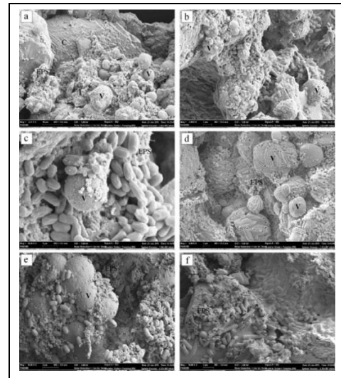
Figure 3. The SEM images of precipitated \text{CaCO}_3 in B. aerius . (a): Calcite (c): vaterite (V) and amorphous formations (EPS), (b-e): Cells formed bacillus (1µm) vaterite and polymeric formations, (f): Cell colonies.
