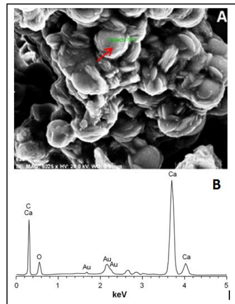
Figure 4. SEM-EDX analysis of precipitated calcium carbonate in S. pasteurii . (A): Vaterite formations. (B): Mass % of elements.
