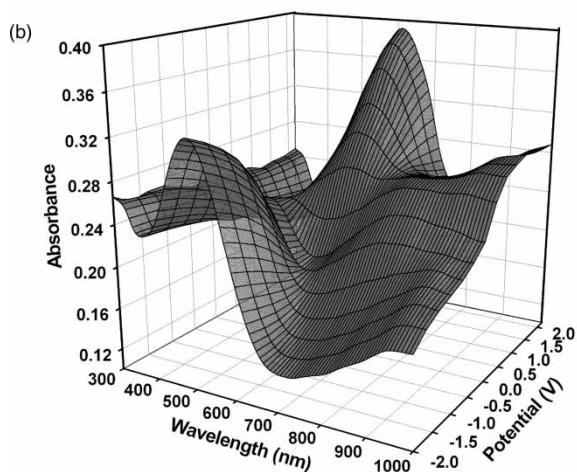
Fig. 9. Series of UV-Vis-NIR absorbance spectra of the P(TPHA-co-EDOT)/PEDOT device under various applied voltages (a) 2D, (b) 3D.
