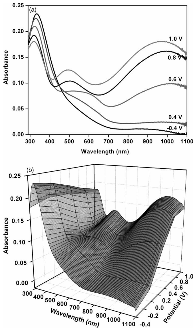
Fig. 3. Optoelectrochemical spectrum of P(TPHA) in the presence of 0.1 M LiClO 4 in AN (a) 2D, (b) 3D.
