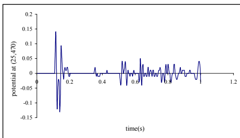
Figure 3i. Potential \phi versus time; for point (25.470) with \beta^1 = 0.6 , \beta^2 = 1.5 , (\Delta x)_1 = 10 m, (\Delta x)_2 = 4 m
