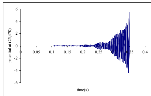
Figure 3d. Potential \phi versus time; for point (25,470) with \beta^1 = \beta^2 = 0.15 , (\Delta x)_1 = (\Delta x)_2 = 5\text{ m}
