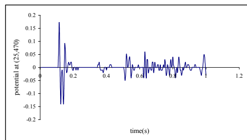
Figure 3f. Potential \phi versus time; for point (25,470) with \beta^1 = \beta^2 = 1.2 , (\Delta x)_1 = (\Delta x)_2 = 5\text{ m}
