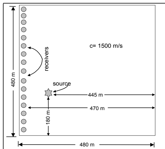
Figure 1. Physical the geometry of the medium used to generate seismograms in the scalar BEM program
