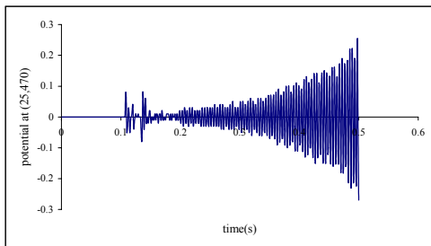
Figure 3h. Potential \phi versus time; for point (25.470) with \beta^1 = 0.15 , \beta^2 = 0.375 , (\Delta x)_1 = 10 m, (\Delta x)_2 = 4 m
