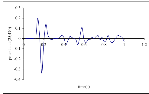
Figure 3c. Potential \phi versus time; for point (25,470) with \beta^1 = 6. , \beta^2 = 15. , (\Delta x)_1 = 5\text{ m} , (\Delta x)_2 = 2\text{ m}
