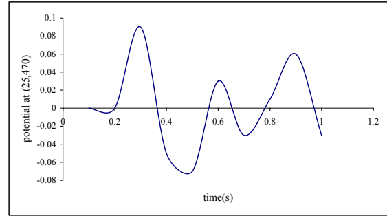
Figure 3j. Potential \phi versus time; for point (25.470) with \beta^1 = 15. , \beta^2 = 37.5 , (\Delta x)_1 = 10 m, (\Delta x)_2 = 4 m
