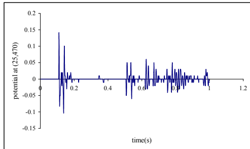
Figure 3e. Potential \phi versus time; for point (25,470) with \beta^1 = \beta^2 = 0.6 , (\Delta x)_1 = (\Delta x)_2 = 5\text{ m}
