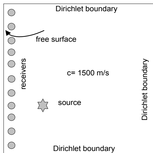
Figure 2. Definition of the boundary conditions of the problem
