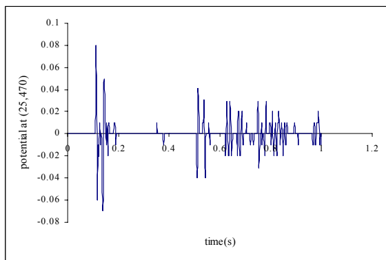
Figure 3b. Potential \phi versus time; for point (25,470) with \beta^1 = 0.6 , \beta^2 = 1.5 , (\Delta x)_1 = 5\text{ m} , (\Delta x)_2 = 2\text{ m}
