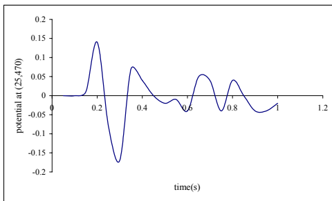
Figure 3g. Potential \phi versus time; for point (25.470) with \beta^1 = \beta^2 = 15. , (\Delta x)_1 = (\Delta x)_2 = 5 m
