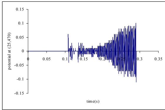
Figure 3a. Potential \phi versus time; for point (25,470) with \beta^1 = 0.15 , \beta^2 = 0.375 , (\Delta x)_1 = 5\text{ m} , (\Delta x)_2 = 2\text{ m}
