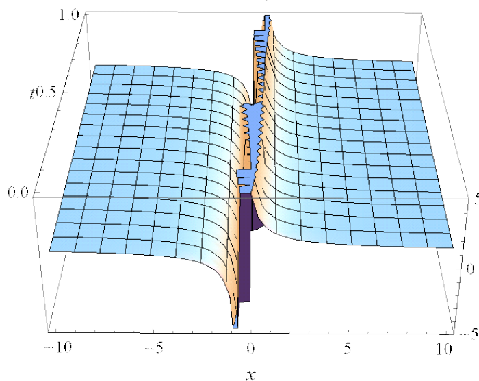
Figure 3: The graphical representation of u_3(x, y, t) for m = 0.1, n = 0.1, \sigma = 0.1, a_0 = 1, \alpha = 0.8, y = 0.5 .
