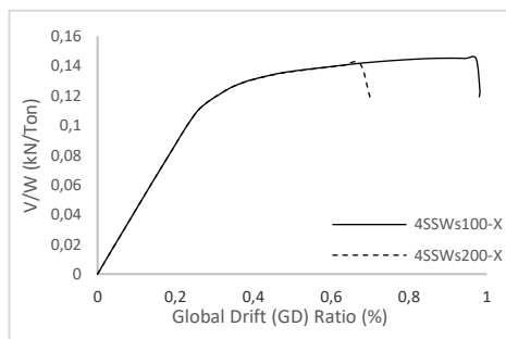
Fig. 5 Capacity curves of 4-story buildings for different transverse reinforcement amount
