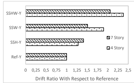
Fig. 7 Average drift demand ratios for ground story at Y axis
