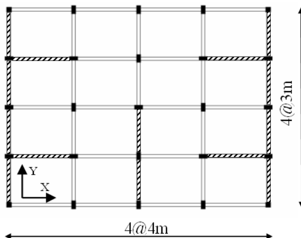
Fig. 1 Plan view of the selected 4- and 7-story buildings
