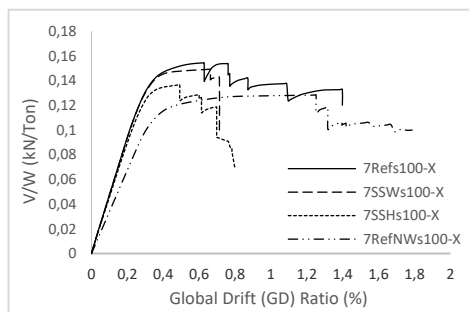
Fig. 4 Capacity curves of 7-story buildings
