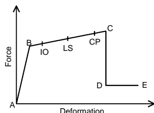
Fig. 2 Force-Deformation relationship of a typical plastic hinge
