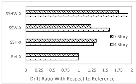
Fig. 6 Average drift demand ratios for ground story at X axis
