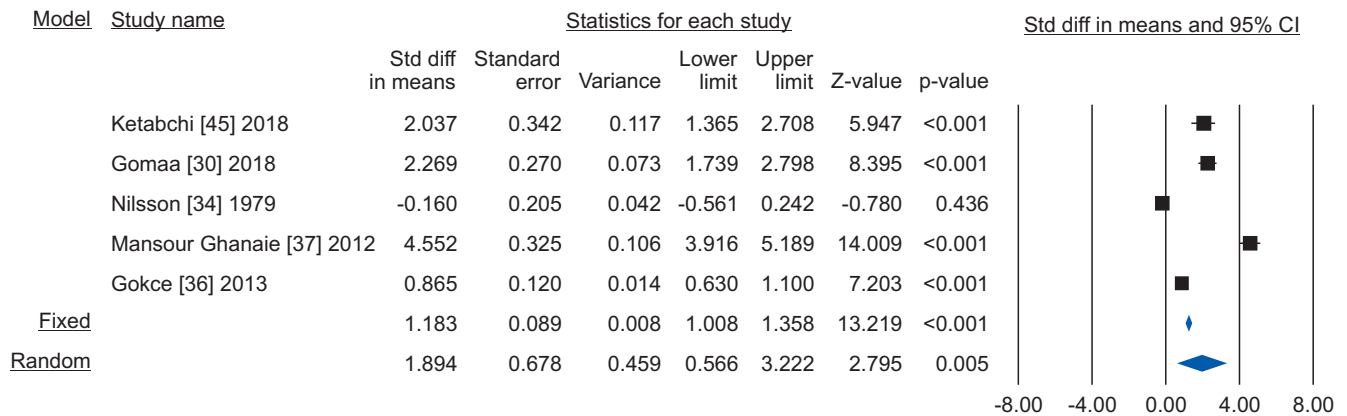
Fig. 10. Forest plot of the total sperm count in infertile men with varicocele repair compared to no treatment.
