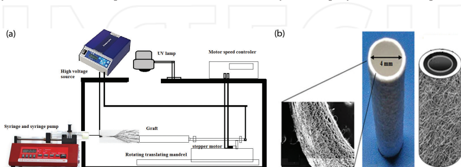
Figure 6. (a) Schematic representation of the reactive electrospinning apparatus with UV light using a rotating mandrel. Modified from Theron et al. [65]. (b) Electrospun vascular graft for regeneration of blood vessel [78].
