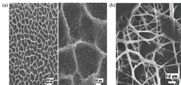
Figure 7. SEM images of self-assembled polyurethane electrospun nanofibers [81]
