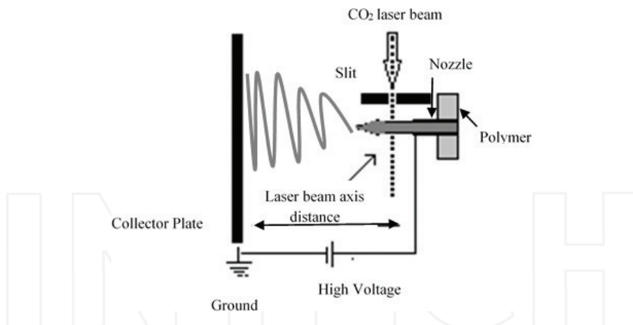
Figure 5. Schematic diagram of laser-electrospinning system. Modified from Takasaki et al. [63].
