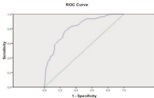
Figure 1 — Receiver operating characteristic curve for posturographic fall risk by fall history. Area under-the-curve: 0.818
