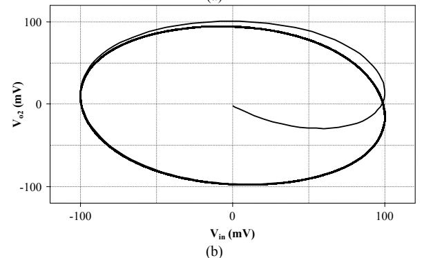
Fig. 11. Lissajous patterns showing (a) +90^\circ phase shift of V_{o1} and (b) -90^\circ phase shift of V_{o2} against input voltage at 9.44 MHz
