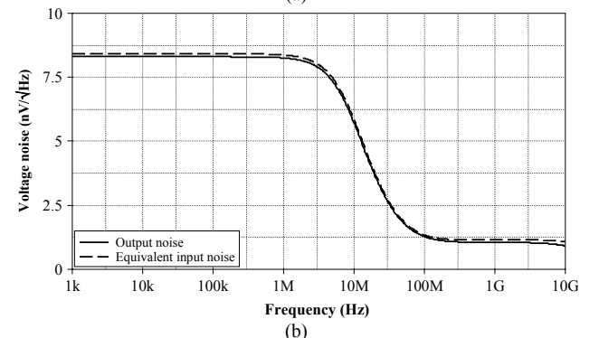
Fig. 8. Input and output noise variations for (a) V_{o1} and (b) V_{o2} versus frequency
